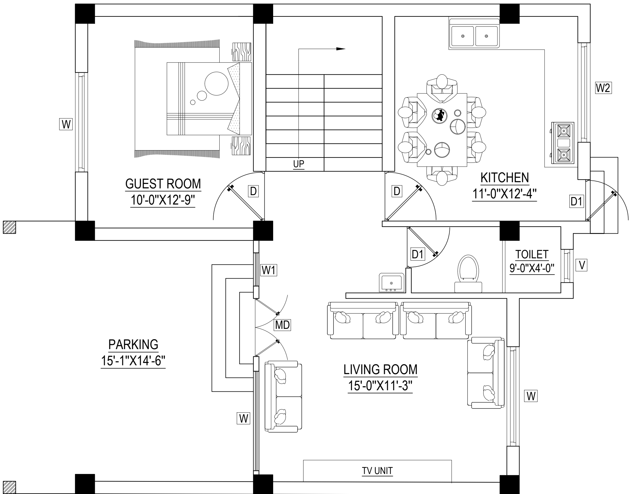
GROUND FLOOR PLAN COUNTABLE AREA=861.00 SQ.FT. UNCOUNTABLE AREA=71.00 SQ.FT. TOTAL AREA=932.00 SQ.FT.
